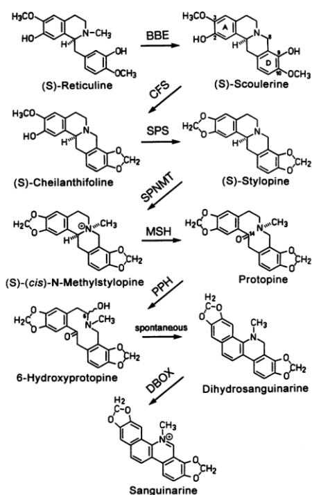
شکل ۱- مسیر بیوسنتزی تولید سنگوئینارین از اس- رتیکولین (Blechert et al. 1995) BBE: Berberine bridge enzyme; CFS: (S)-cheilanthifoline synthase; SPS: (S)-stylophine synthase; SPNMT: S-adenosyl-L-methionine: (S)-tetrahydroprotoberberine cis-N-methyltransferase; MSH: (S)-cis-N-methylstylophine 14-hydroxylase; PPH: protopine 6-hydroxylase; DBOX: (dihydrobenzophenanthridine oxidase)
